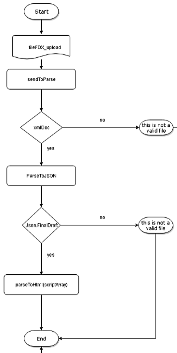
Figure 2. Flowchart parsing algorithm
