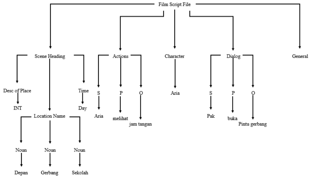
Figure 3. Parse tree
