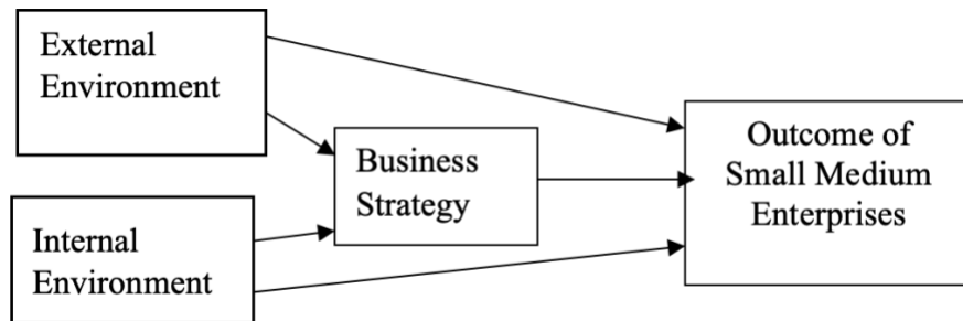
Figure 2. Research Framework
